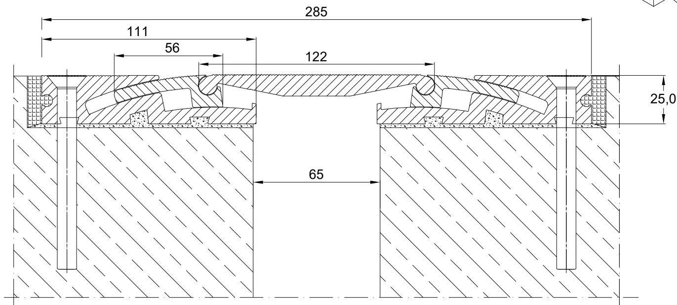
CONECTO HDS 285.30.25 SECTION
